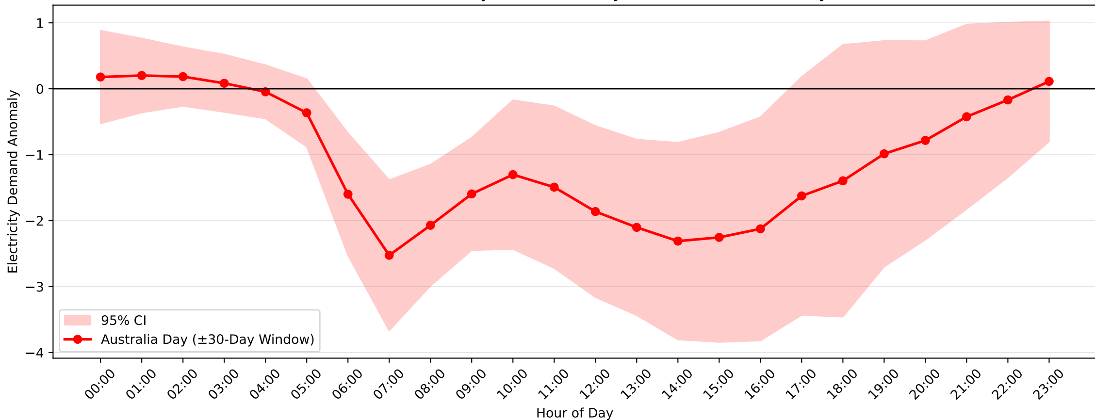
Five Dock Demand Anomaly: Australia Day (2004–2017, \pm 30 -Day Window)
